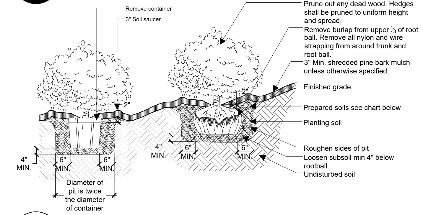
16 Planting Pit for Shrubs L-3.1
