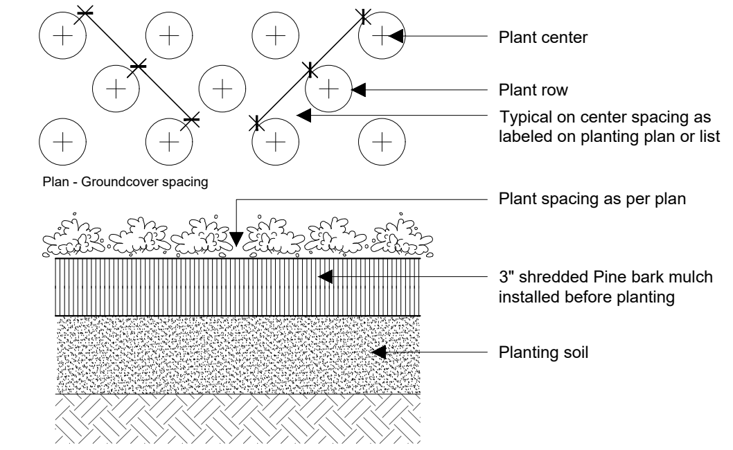
15 Groundcover Planting L-3.1
