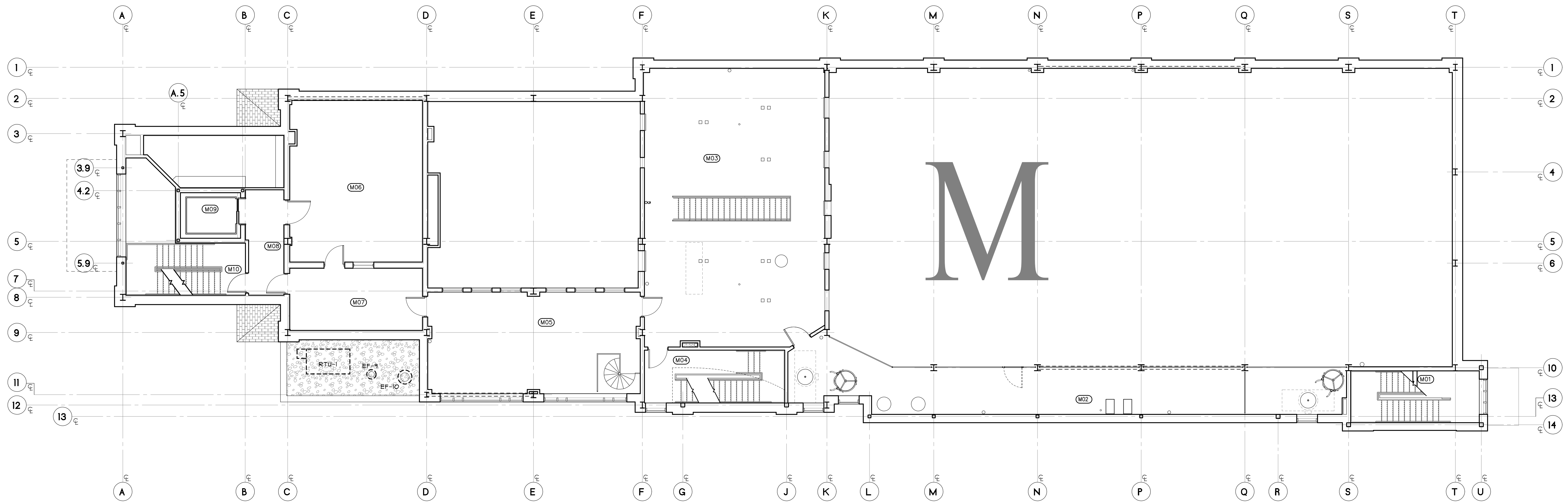
2 MID-LEVEL/MEZZANINE PLAN A1.1 SCALE: 1/8" = 1'-0"
