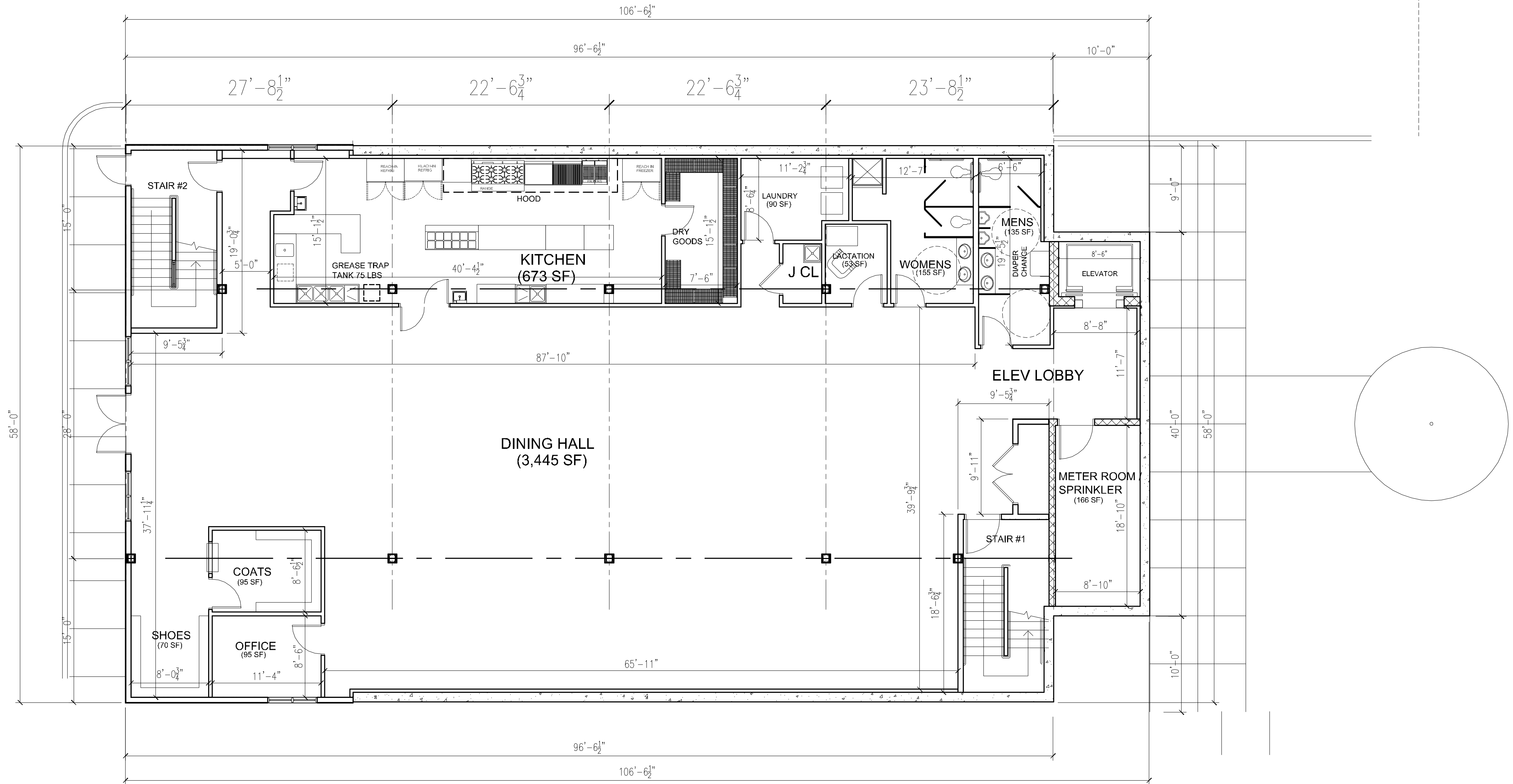
BASEMENT FLOOR PLAN SCALE - 3/16" = 1'-0"
