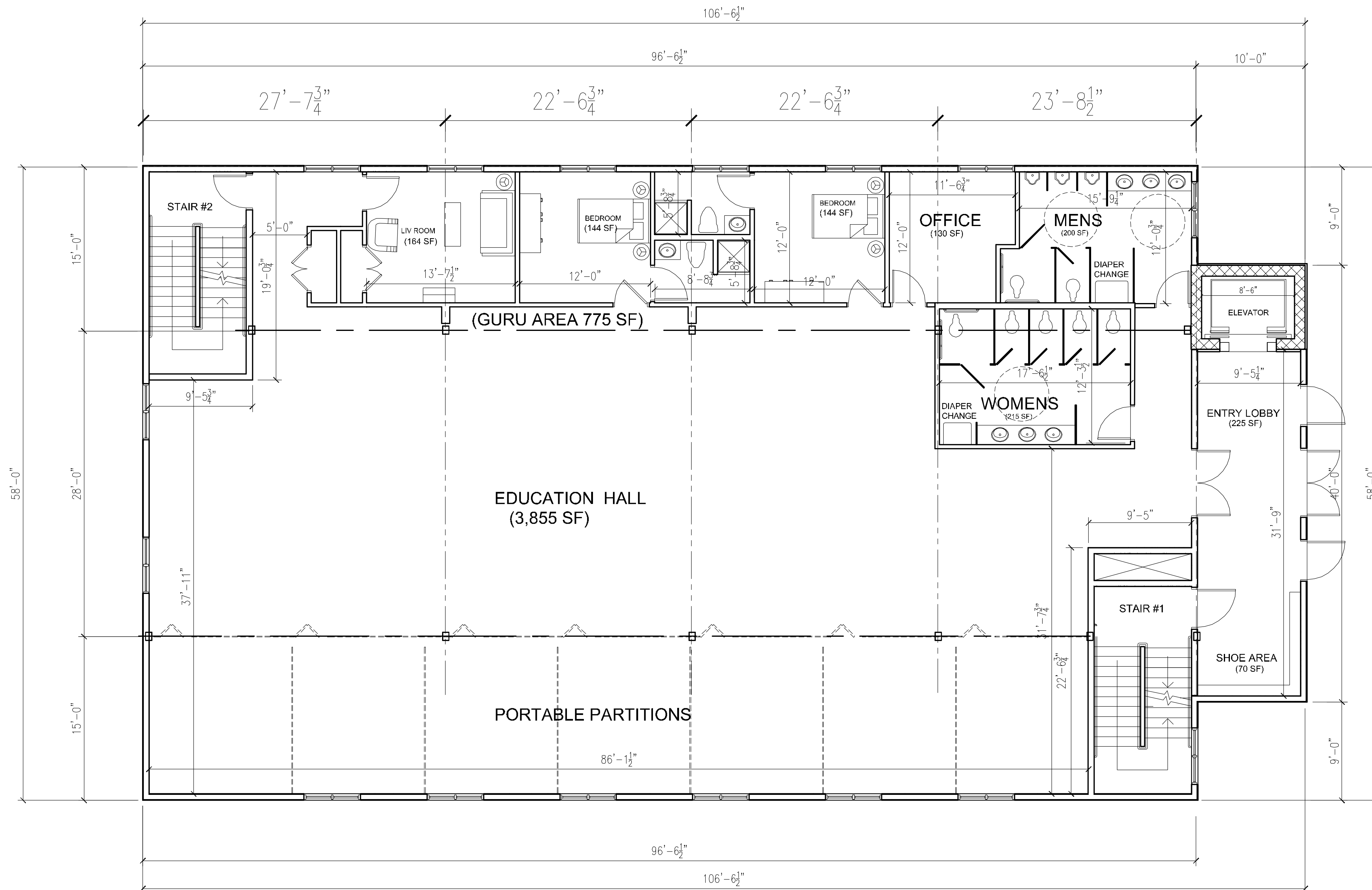
FIRST FLOOR COMMUNITY HALL PLAN SCALE - 3/16" = 1'-0"
